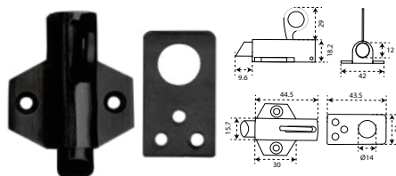
SKP 605 SPRING KNIFE EXCLUSIVE BRASS
