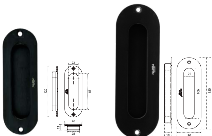
CMP 220 OVAL 12CM
