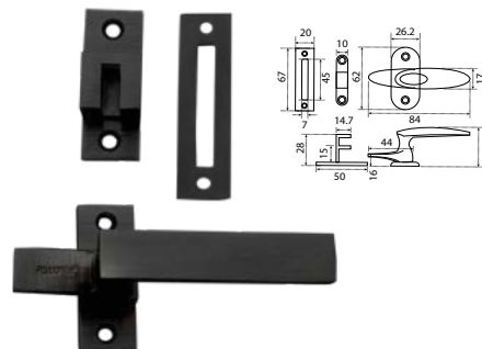
RBP 665 RAMBUNCIS ORLANDO BRASS
