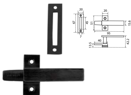
RBP 685 RAMBUNCIS BOSTON BRASS
