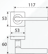
HRP 5404 HOPE SQ ZZ - ZAMAK 3
