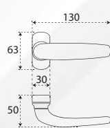
HRP 5405 MARTIN SQ ZZ - ZAMAK 3
