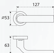
HRP 5403 WINA ZZ - ZAMAK 3
