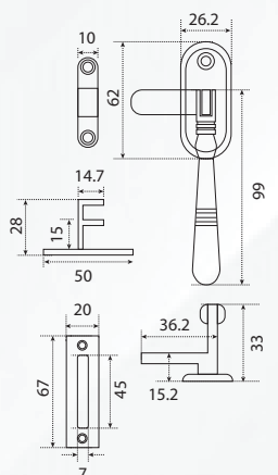
RBP 625 LUNA - BRASS
