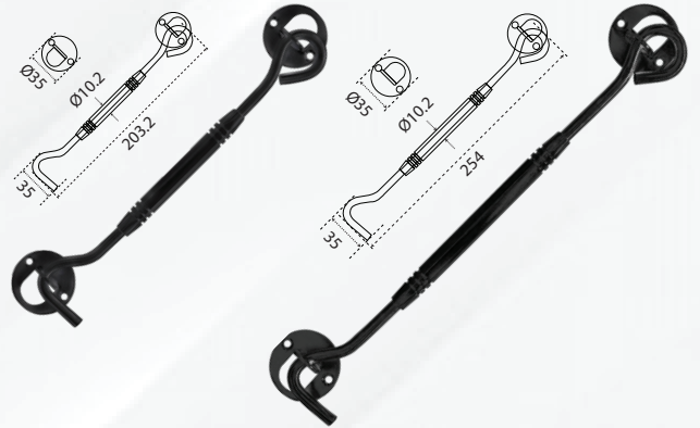
WHP 509 501-8" SG6 - STEEL
